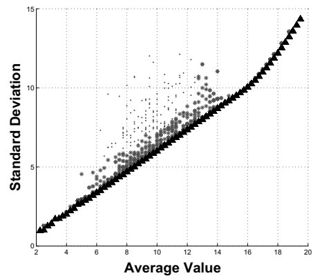
(b) Result for Motorola Data Set
