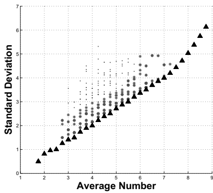
(b) Result for Motorola Data Set
