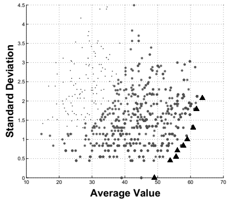
(c) Result for Greer Data Set
